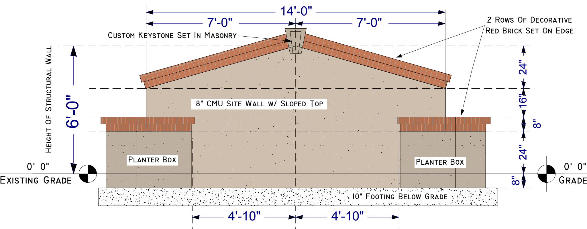
H.O.A. ENTRY SIGN ELEVATION
